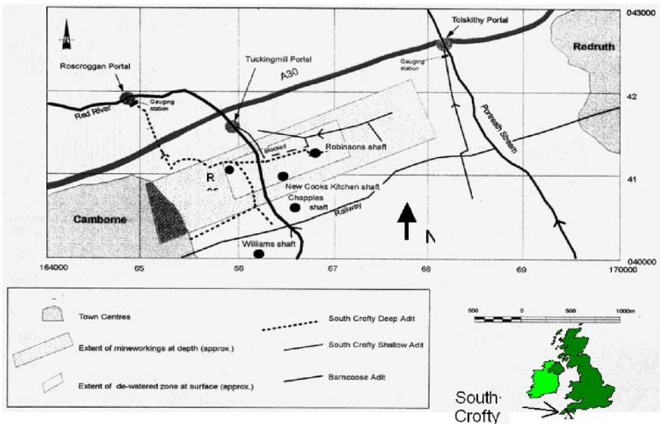
Figure 1 Location map of South Crofty Mine, showing the extent of the modern workings, principal shafts and drainage adits.
