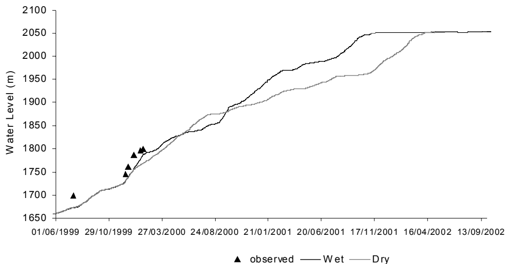
Figure 4 Modelled water levels in Roskear Shaft from June 1999 until emergence of mine water in Dolcoath Adit, under wet and dry recharge scenarios.
