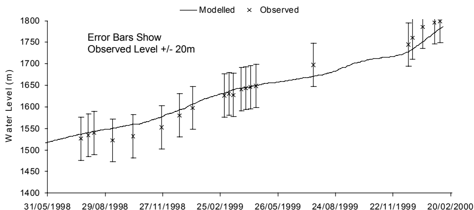
Figure 3 Observed and modelled water levels in Cooks Kitchen Shaft from June 1998 to January 2000.
