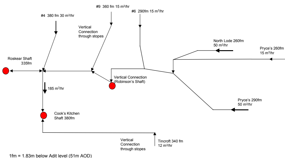
Figure 2 Schematic diagram of modelled inflows and the pipe network included in the conceptual model, depicting flow rates and location (by mined level).
